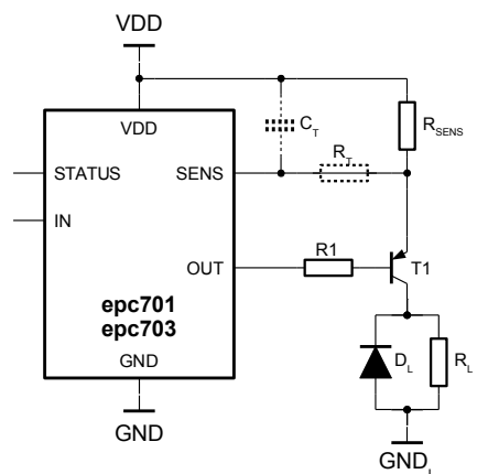
Figure 7: epc701 or epc703 using an external switching transistor. In case of a short-circuit in the load the turn-off delay can be extended by an external RC network. This network adds t_{\text{ext}} to the internal delay t_{\text{del}} .
