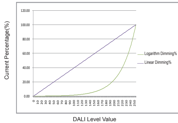
DALI Curve
