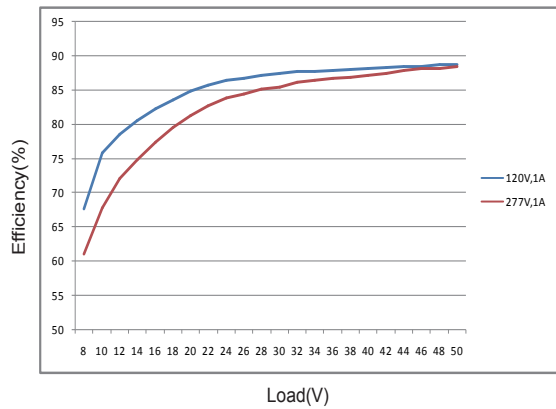
Efficiency Curve
