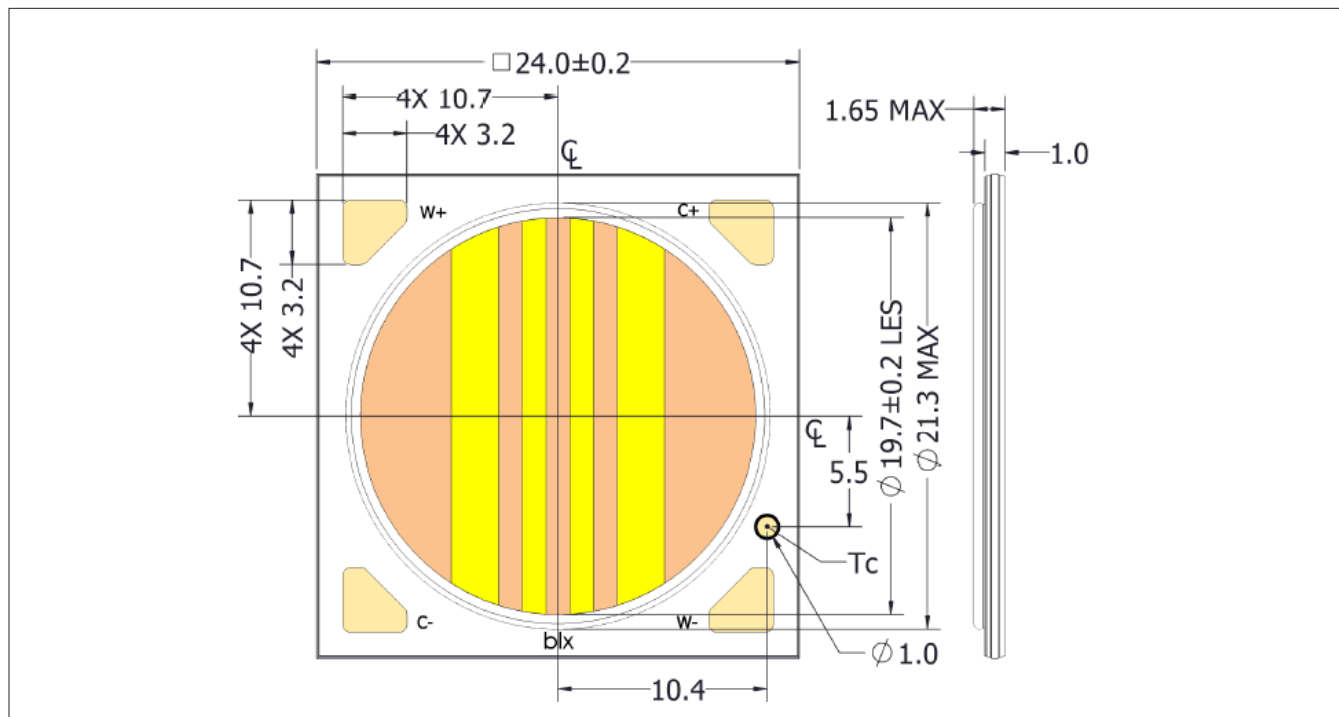
Figure 14: Drawing for Vesta Series Tunable White Gen 2 18mm Array
