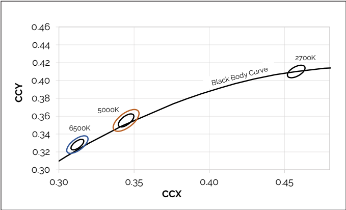
Figure 15: Graph of Bins in xy Color Space
