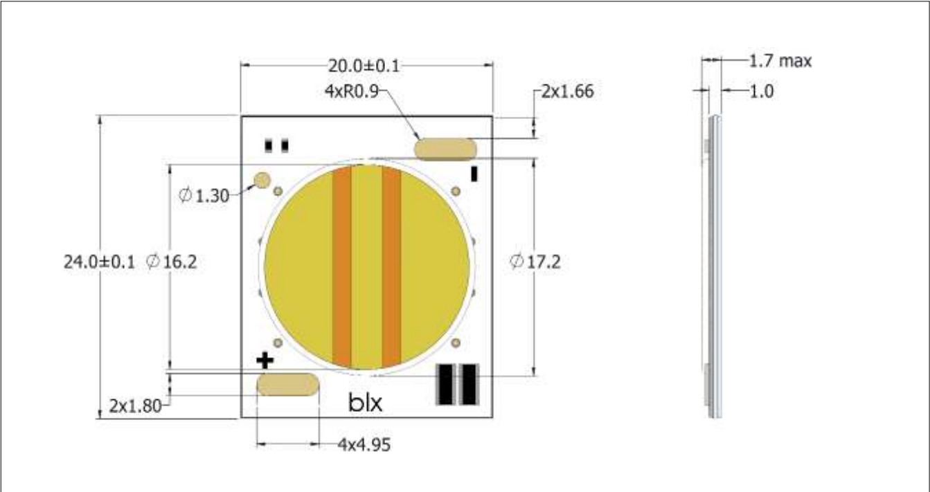
Figure 11: Drawing for Vesta Series Dim-To-Warm 15mm Array
