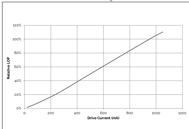
Figure 3: Vesta Dim-to-Warm 15mm 33W Relative LOP vs. Drive Current, T_c = 25^\circ\text{C}
