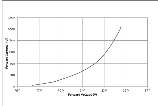
Figure 1: Vesta Dim-to-Warm 15mm 33W Forward Voltage vs. Forward Current, T_c = 25^\circ\text{C}
