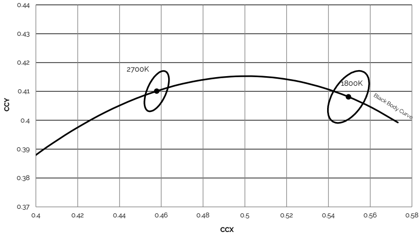
Figure 12: Graph of Warm White Test Bins in xy Color Space, T_c = 25^\circ\text{C}
