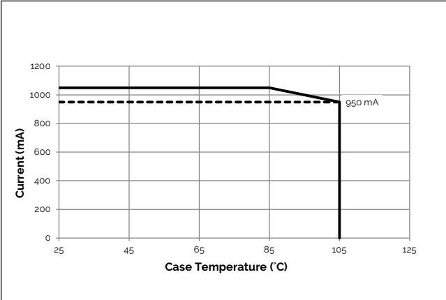
Figure 7: Vesta Dim-to-Warm 15mm 33W Derating Curve
