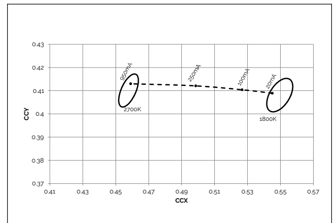
Figure 4: Vesta Dim-to-Warm 15mm 33W Color Shift vs. Forward Current 2700K-1800K
