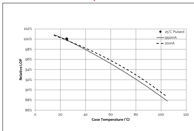
Figure 5: Vesta Dim-to-Warm 15mm 33W Relative Flux vs. Case Temperature
