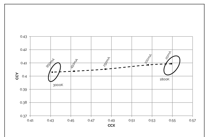
Figure 6: Vesta Dim-to-Warm 15mm 33W Color Shift vs. Forward Current 3000K-1800K
