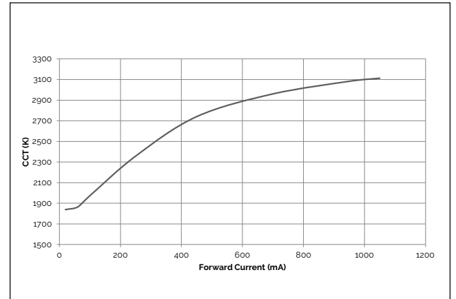
Figure 2: Vesta Dim-to-Warm 15mm 33W CCT vs. Forward Current
