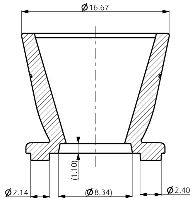
SECTION B-B
