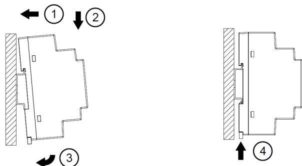
Fig. 2.1 Mounting
