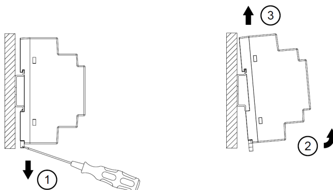
Fig. 2.2 Dismounting
