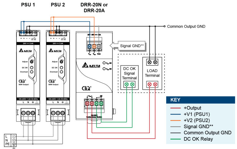
Fig. 9 Redundant Operation Connection Diagram
