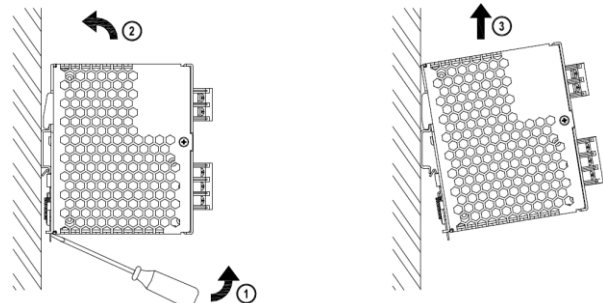
Fig. 2.2 Dismounting
