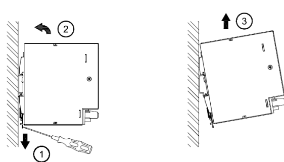
Fig. 2.2 Dismounting
