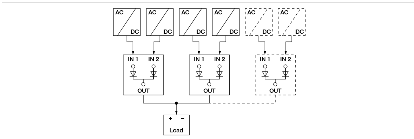
Fig. 3.3 N+1 Redundancy
