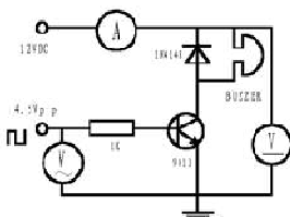
Test Circuit
