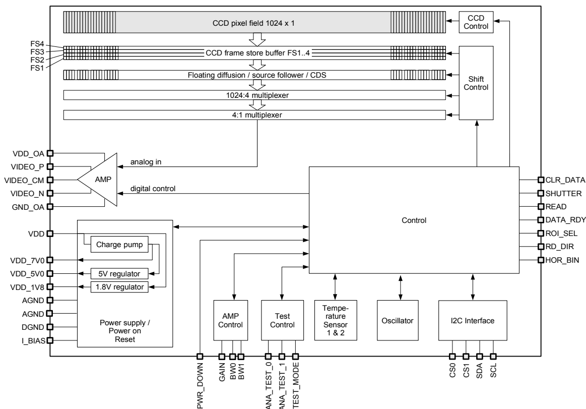
Figure 3: Block diagram
