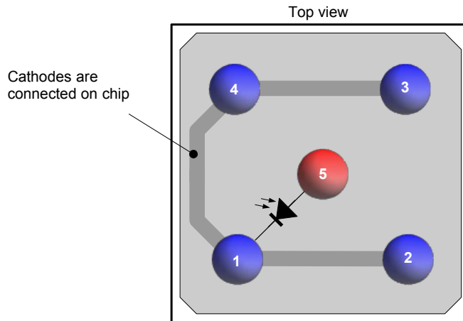
Figure 6: Pin-out
