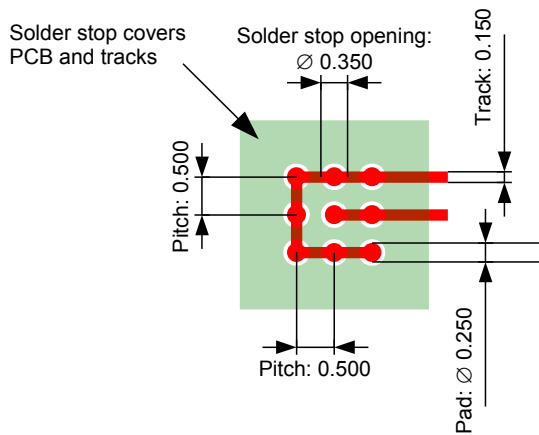
Figure 8: Recommended PCB layout (all measures in mm)
