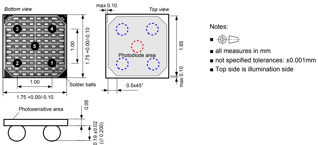
Figure 7: Dimensions epc200-CSP5
