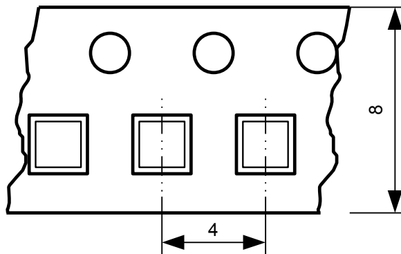
Figure 9: Tape dimensions (all measures in mm) Note: Solder balls are bottom side
