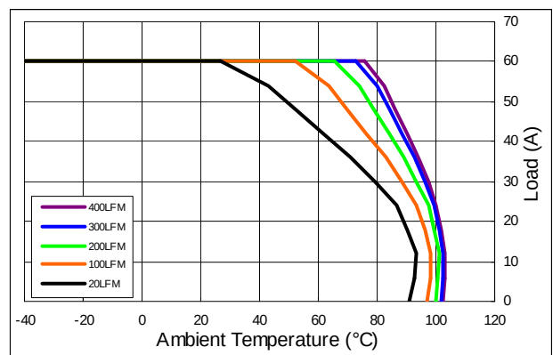
Derating curves of CBH48015abcA-60XXX for T C =110°C
