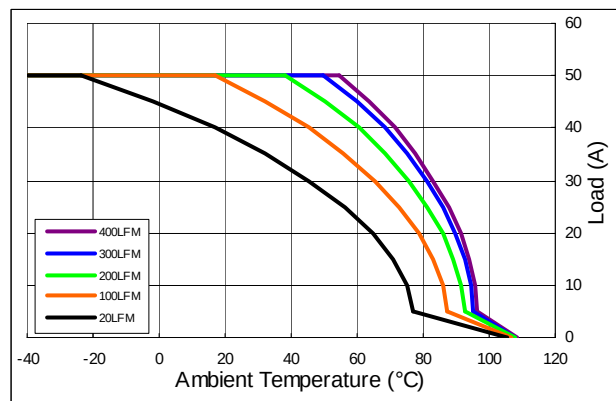
Derating curves of CBH24050abcA-50XXX for T C =110°C
