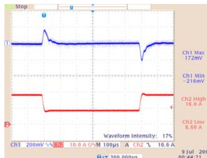
Transient response of CPH48033abcd-70XXX ( V_{IN} : 48V, Load: 18A/8A@2.5A/µs)
