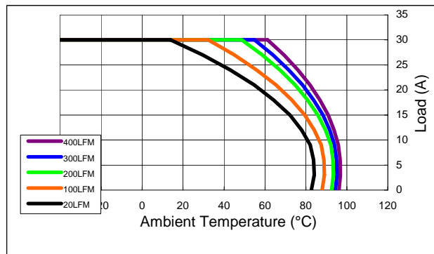
Derating curves of COE48033abcA-30XXX for T_C=110^{\circ}C
