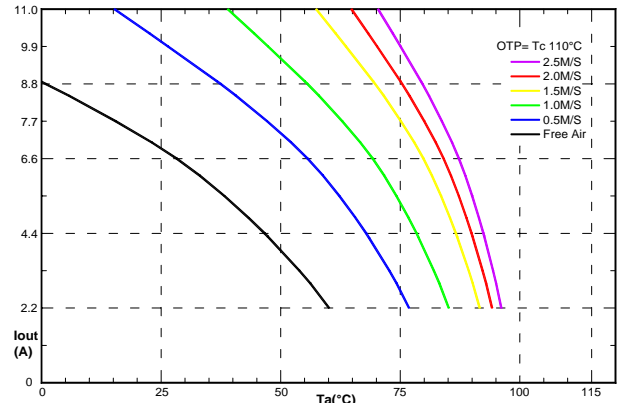
Derating curves of COE48120abcA-11XXX for T_C = 110^\circ\text{C}
