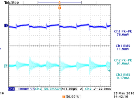
Input/Output ripples of COE48120abcd-11XXX ( V_{IN} : 48V, Load: 11A, L_{IN} =10uH)
