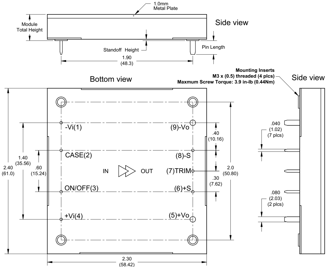
Dimensions and Pin Connections
