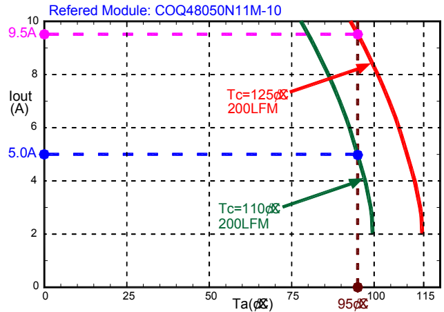
Plot-1: Derating curves for Tc=110°C and Tc=125°C
