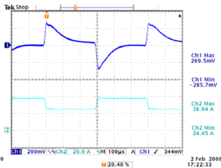
Transient response of UH48120abcd-N50xxx ( V_{IN} : 48V, Load: 38.0A/25.0A@2.5A/μs)
