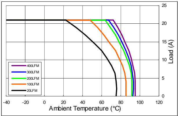
Derating curves of UQ48120abcB-21XXX for T_C = 110^\circ C
