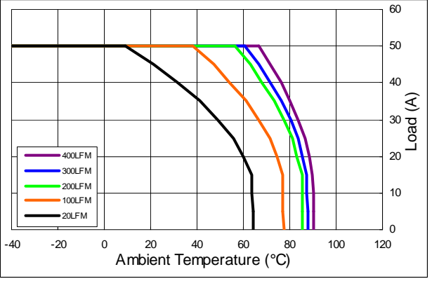
Derating curves of UQ48050abcB-50XXX for T_C = 110^\circ C
