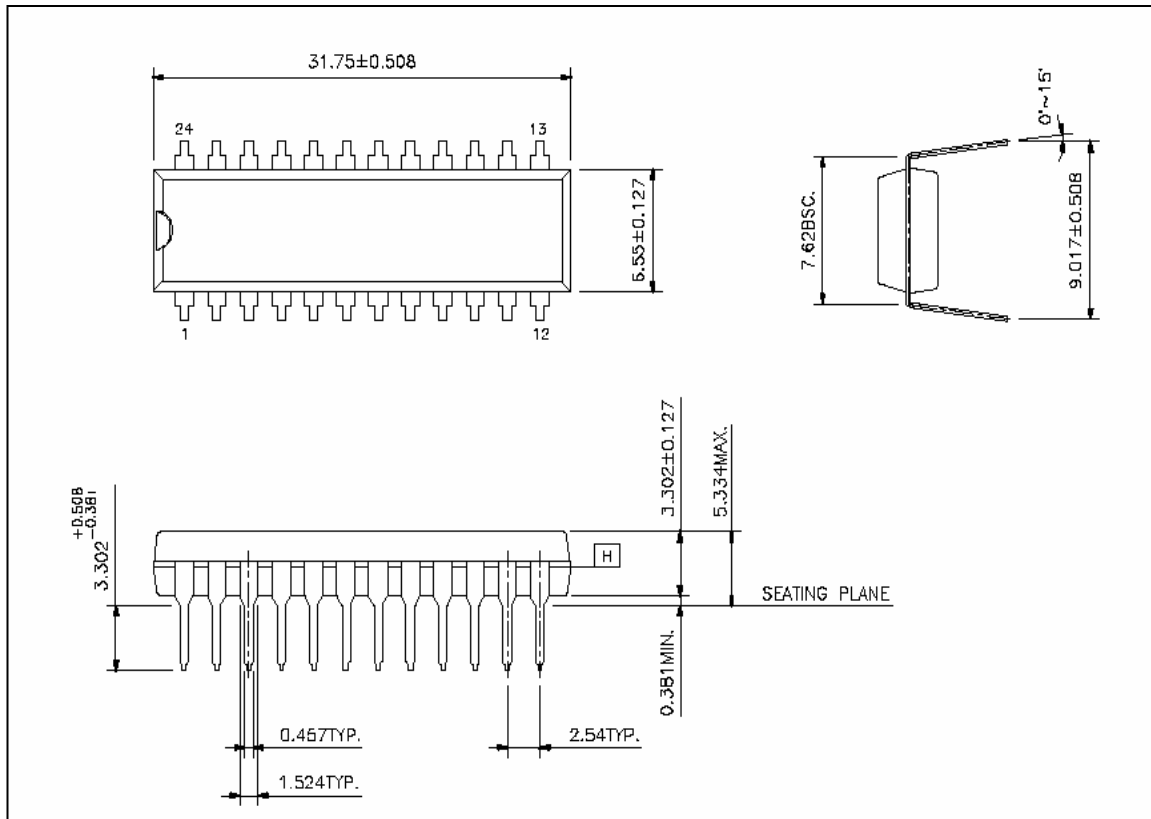
MBI5029CN\GN Outline Drawing
