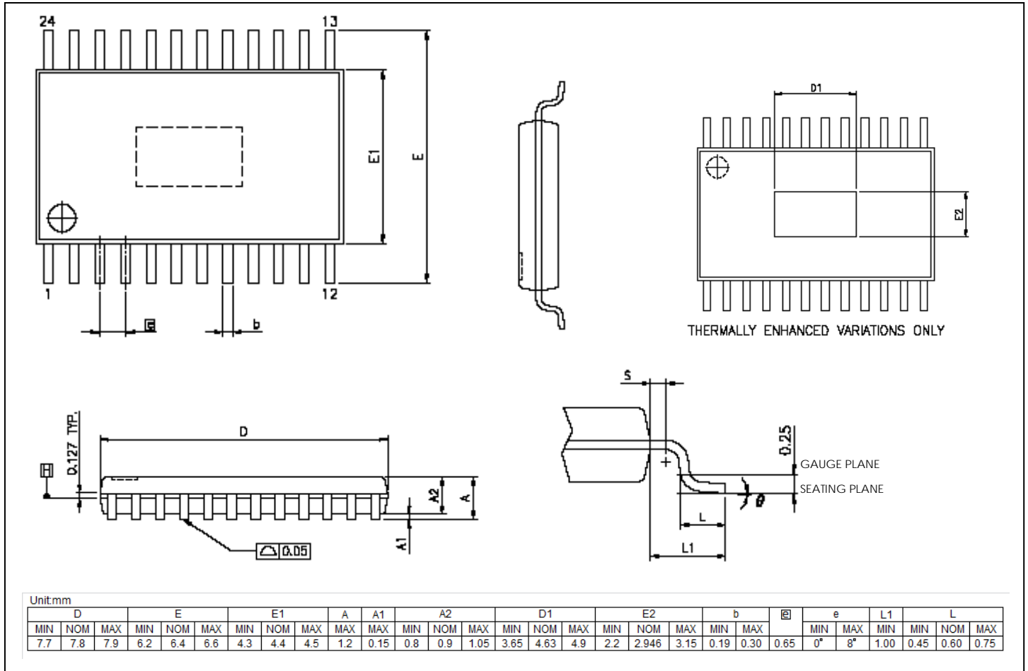
MBI5040 GTS Outline Drawing
