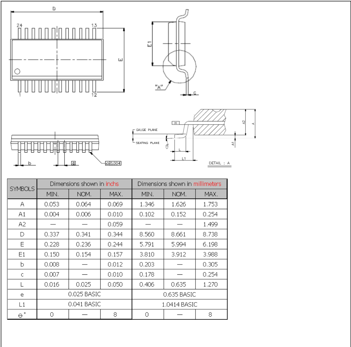
MBI5040GP Outline Drawing
