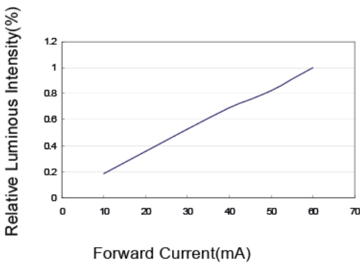
Fig.2 Forward current vs. Luminous Intensity
