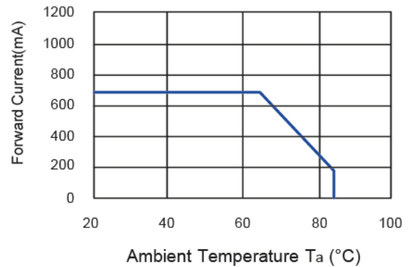
Fig.2 Forward Current VS. Ambient Temperature
