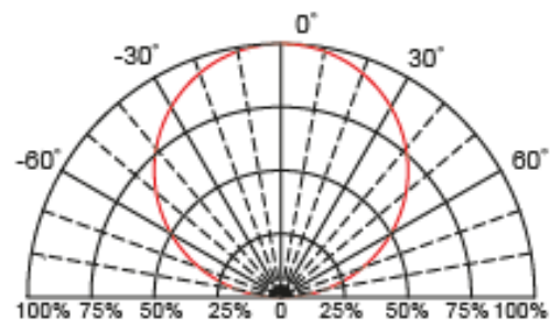
Fig.6 Directive Radiation
