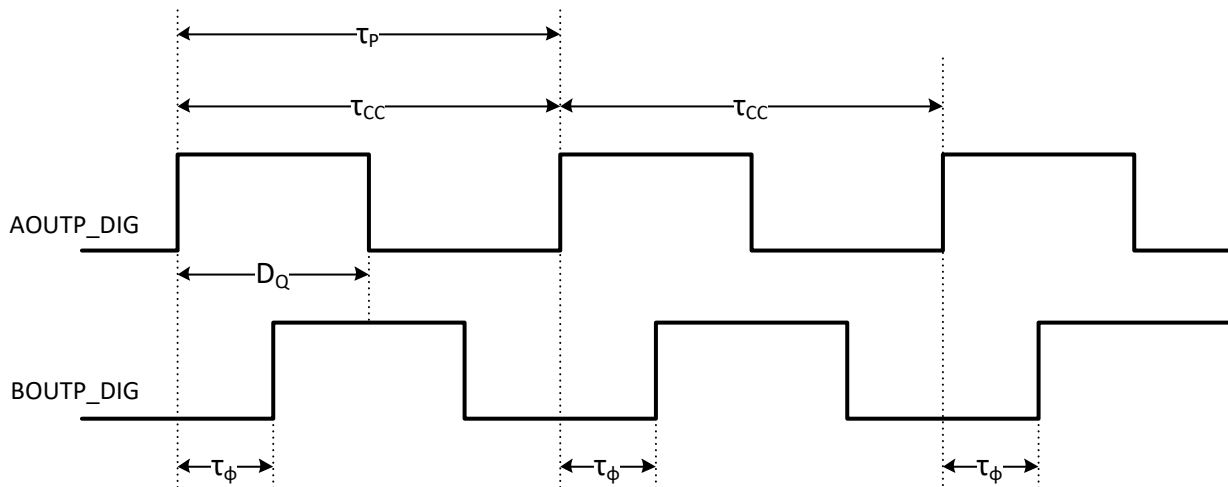
Figure 3: Jitter specification diagram; with \tau_p as time period, \tau_{CC} as a similar time used to calculate cycle-to-cycle jitter, D_Q as the duty cycle, and \tau_\phi as time of the phase difference between A and B. The phase error, \epsilon_\phi , can be calculated as 360(\tau_\phi/\tau_p) .
