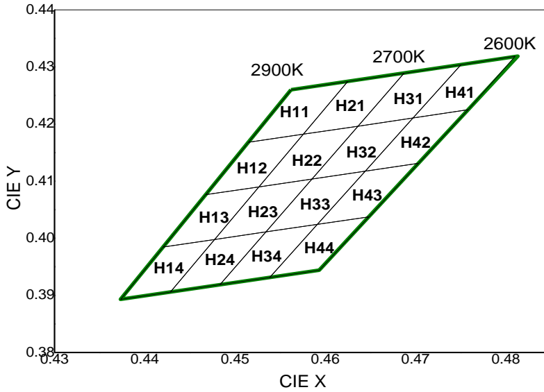
CIE Chromaticity Diagram (Warm white), T_j=25^\circ\text{C} , I_F=75\text{mA}
