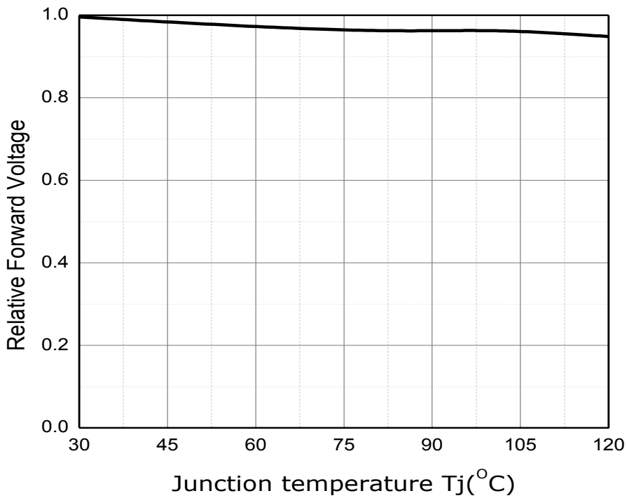
Fig 7. Junction Temperature vs. Relative Forward Voltage, I_F=75\text{mA}
