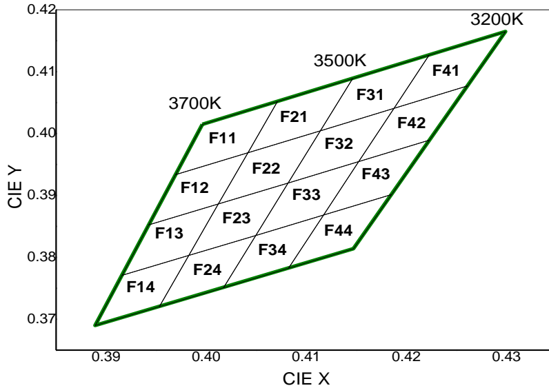
CIE Chromaticity Diagram (Warm white), T_j=25^\circ\text{C} , I_F=75\text{mA}
