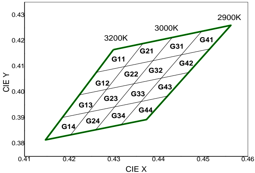
CIE Chromaticity Diagram (Warm white), T_j=25^\circ\text{C} , I_f=75\text{mA}
