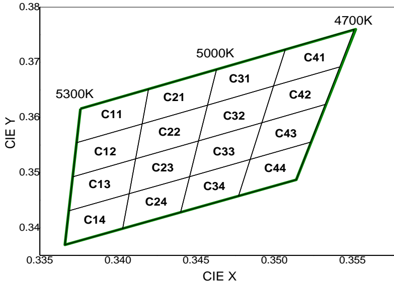
CIE Chromaticity Diagram (Cool white), T_j=25^\circ\text{C} , I_f=75\text{mA}
