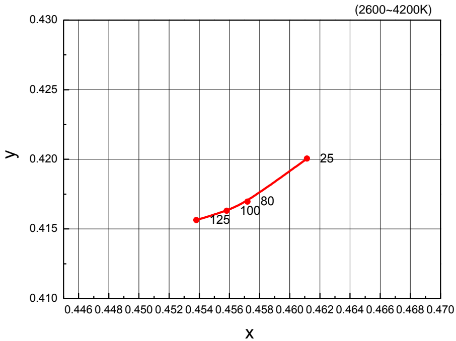
Fig 8. Chromaticity Coordinate vs. Junction Temperature, I_F=75\text{mA}
