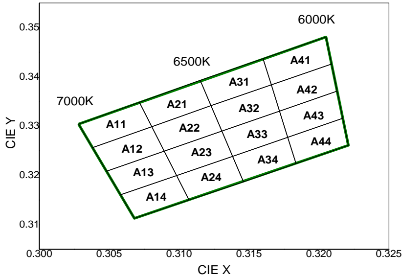
CIE Chromaticity Diagram (Cool white), T_j=25^\circ\text{C} , I_F=75\text{mA}
