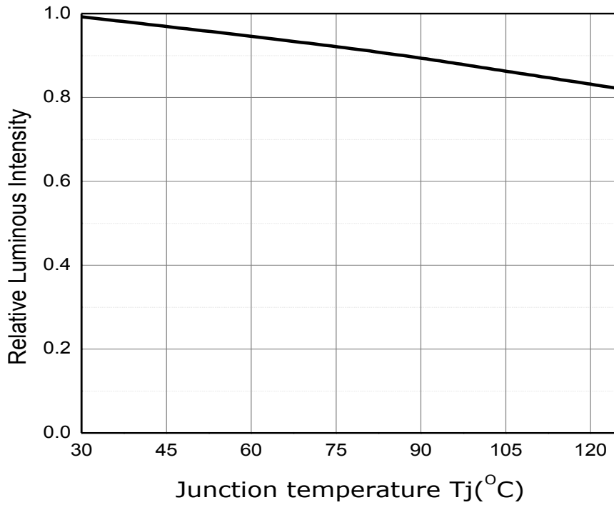
Fig 6. Junction Temperature vs. Relative Luminous Intensity, I_F=75\text{mA}
