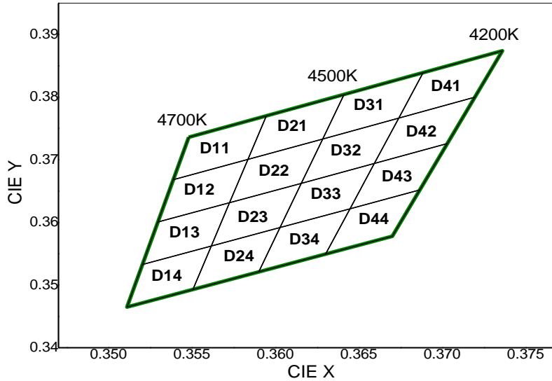
CIE Chromaticity Diagram (Neutral white), T_j=25^\circ\text{C} , I_F=75\text{mA}
