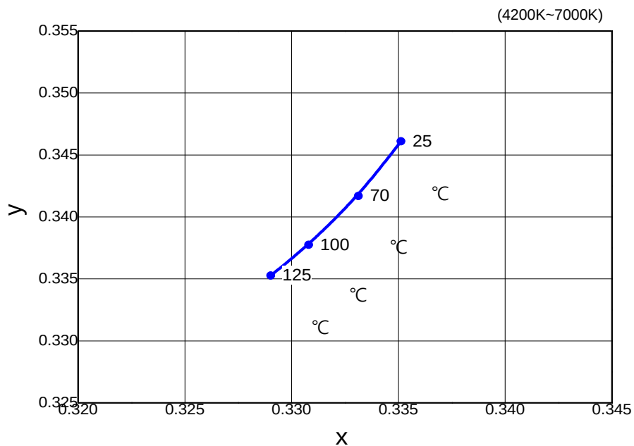
Fig 8. Chromaticity Coordinate vs. Junction Temperature, I_F = 100\text{mA}
