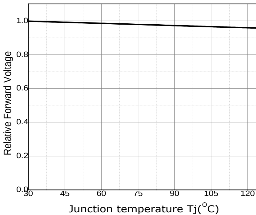
Fig 7. Junction Temperature vs. Relative Forward Voltage, I_F = 100\text{mA}
