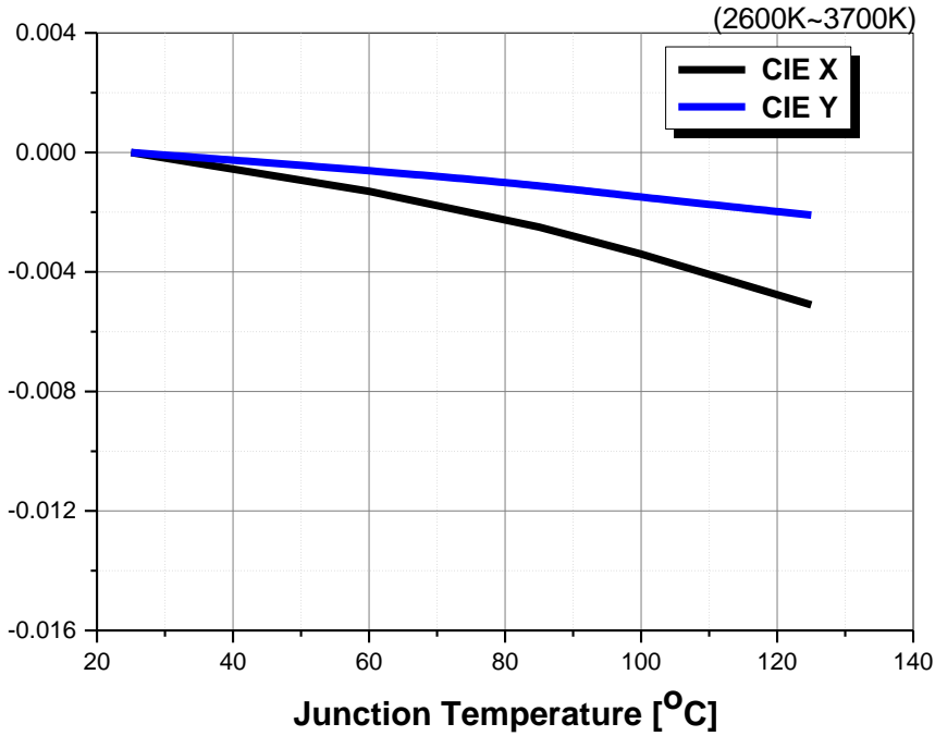
Fig 10. Junction Temp. vs. CIE X, Y Shift, I_F=640mA
