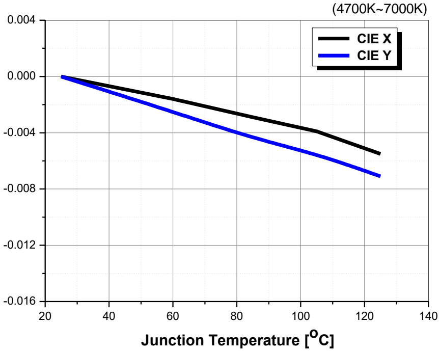
Fig 9. Junction Temp. vs. CIE X, Y Shift, I_F=640\text{mA}
