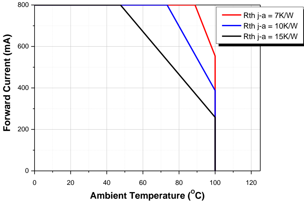
Fig 11. Ambient Temperature vs. Maximum Forward Current, T_{j\_max} = 125^{\circ}\text{C}
