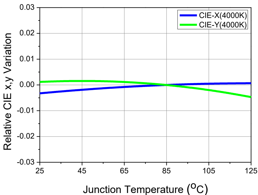
Fig 8. Junction Temperature vs. CIE x,y Shift, I_F=0.29A (4000K)
