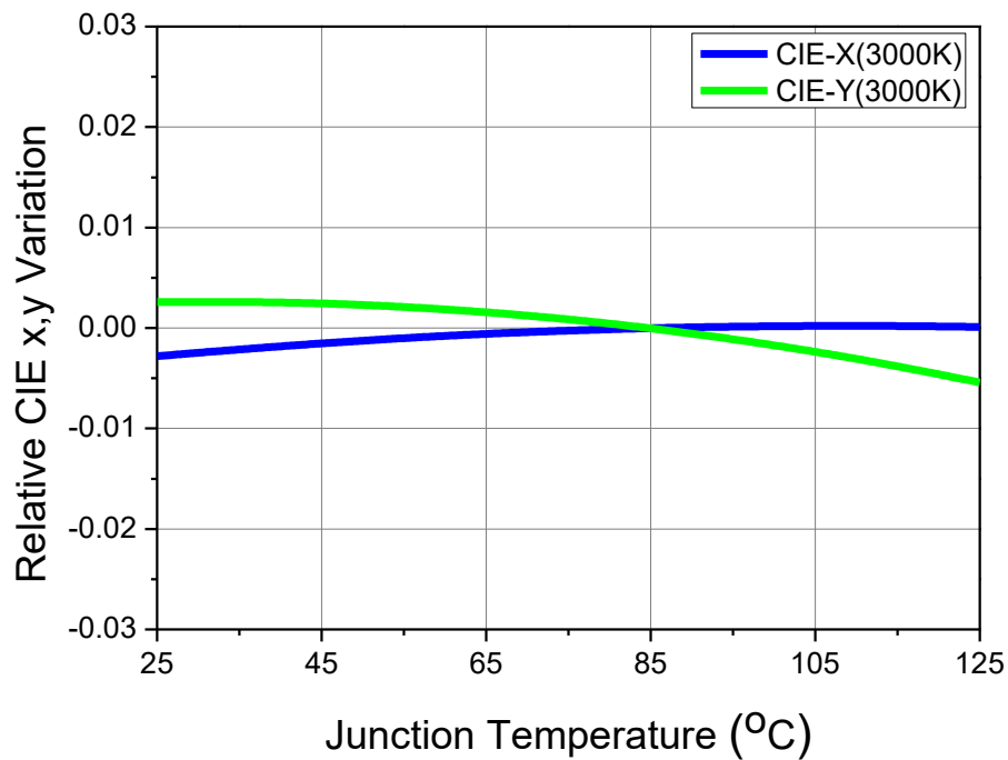
Fig 9. Junction Temperature vs. CIE x,y Shift, I_F=0.29A (3000K)
