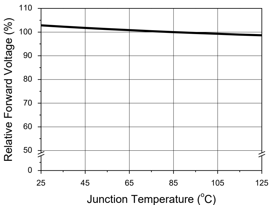
Fig 6. Junction Temperature vs. Forward Voltage, I_F=0.29A
