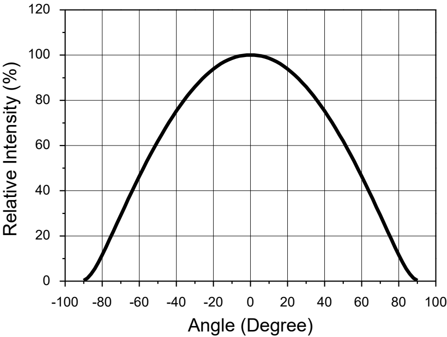
Fig 2. Radiant Pattern
