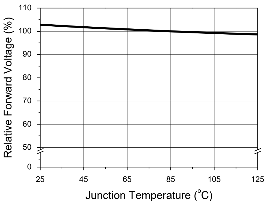
Fig 6. Junction Temperature vs. Forward Voltage, I_F=0.43A
