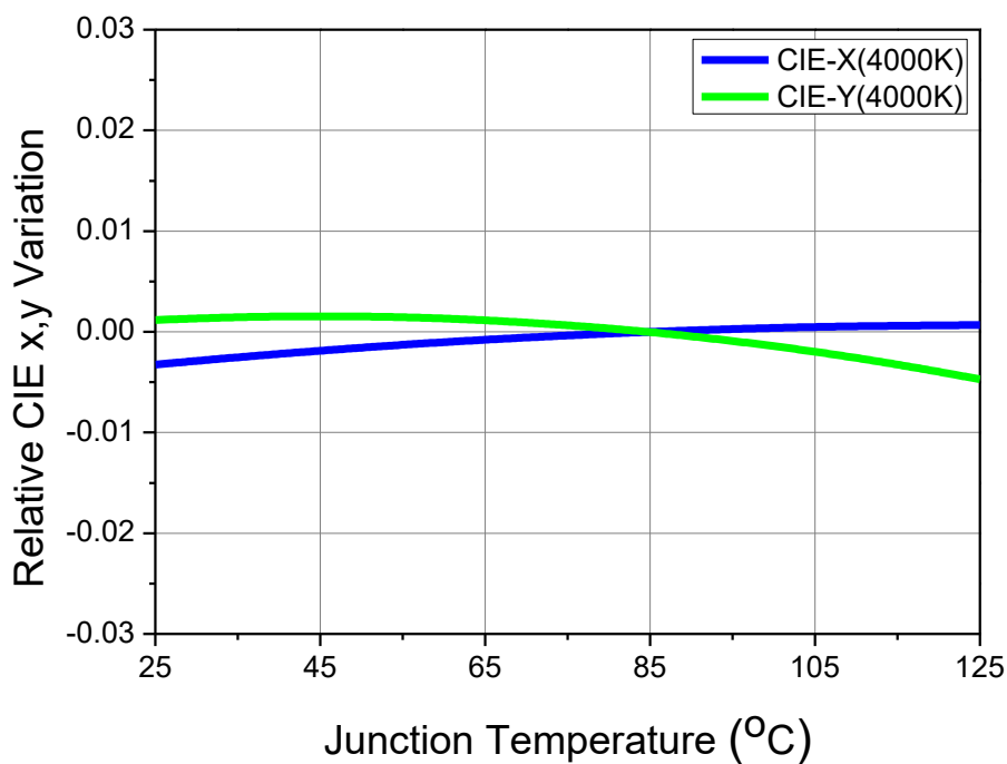
Fig 8. Junction Temperature vs. CIE x,y Shift, I_F=0.43A (4000K)
