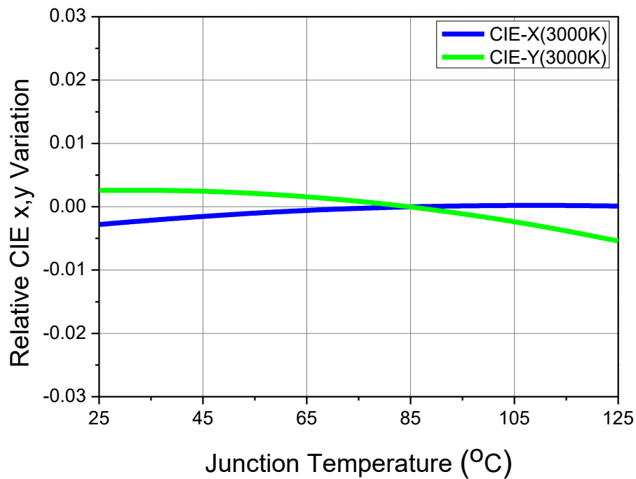
Fig 9. Junction Temperature vs. CIE x,y Shift, I_F=0.43A (3000K)
