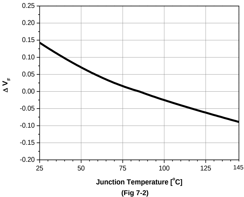
Relative Forward Voltage vs. Junction Temperature, I_F=700\text{mA}
