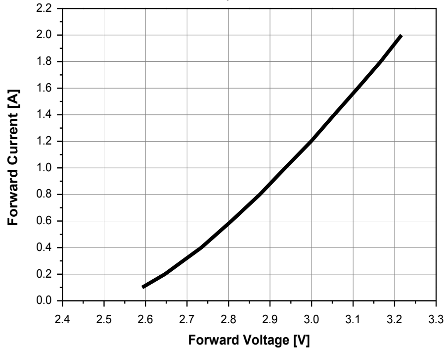
Forward Voltage vs. Forward Current, T_j=85^{\circ}\text{C}
