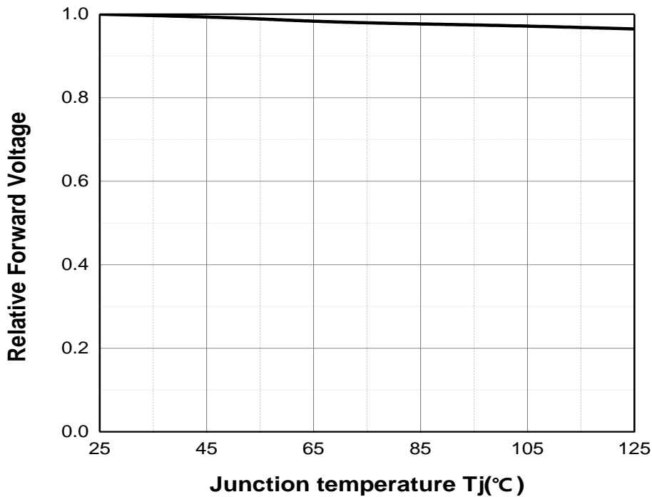
Fig 8. Junction Temperature vs. Relative Forward Voltage, IF=640mA
