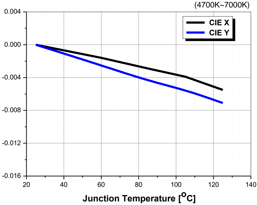
Fig 9. Junction Temp. vs. CIE X, Y Shift, IF=640mA
