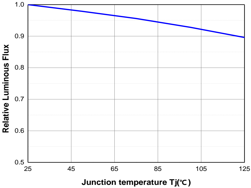
Fig 7. Junction Temperature vs. Relative Luminous Flux, IF=640mA
