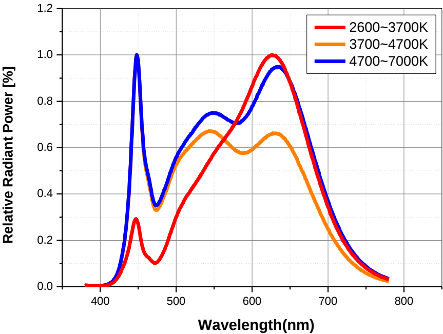
Fig 1. Color Spectrum, T_j = 25^{\circ}\text{C} , I_F = 20\text{mA}
