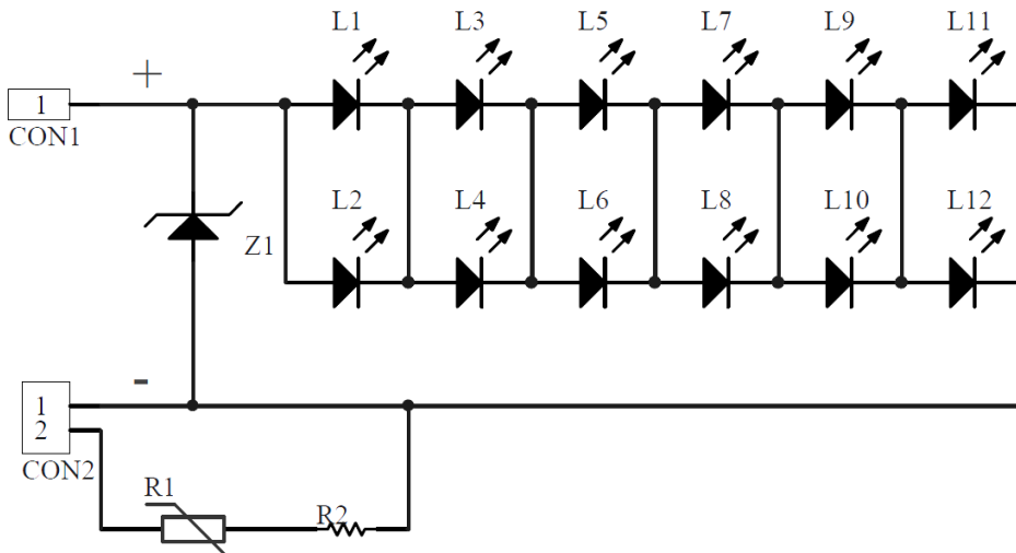
Fig 10. circuit drawing
