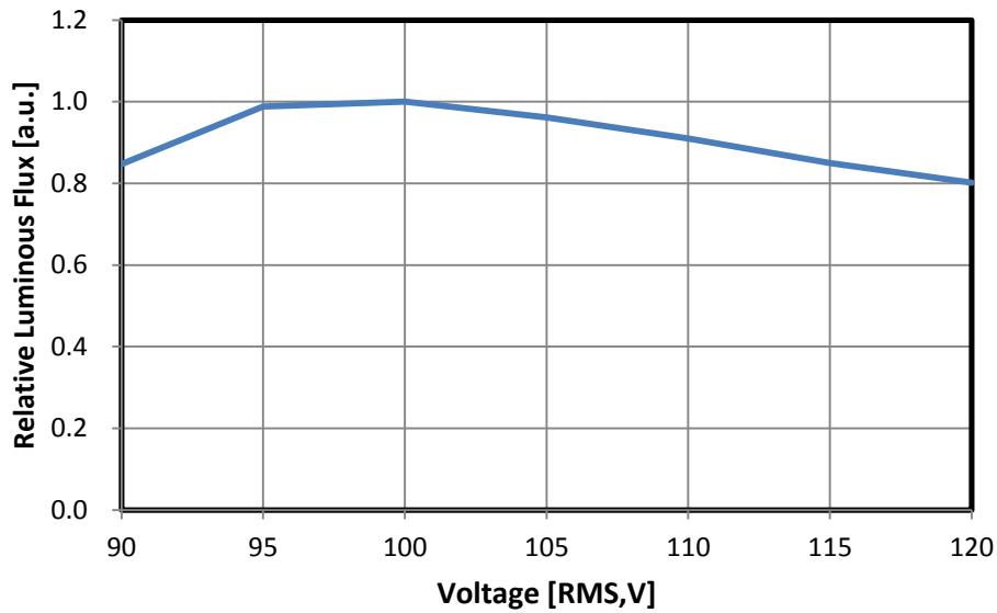
Fig 6. Relative Luminous Flux vs. Voltage, T_a = 25^\circ\text{C} , 120V
