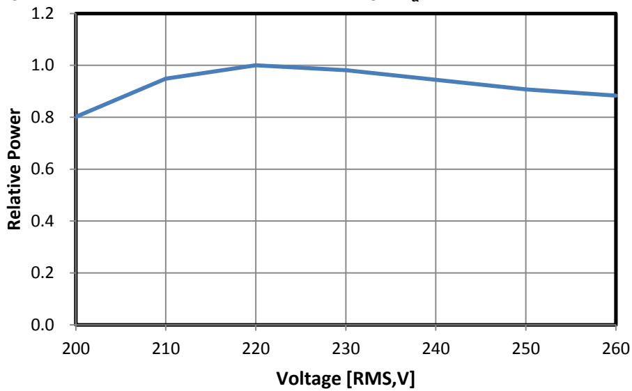
Fig 5. Relative Power Distribution vs. Voltage, T_a=25^{\circ}\text{C} , 220V
