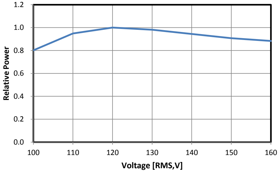
Fig 4. Relative Power Distribution vs. Voltage, T_a=25^{\circ}\text{C} , 120V
