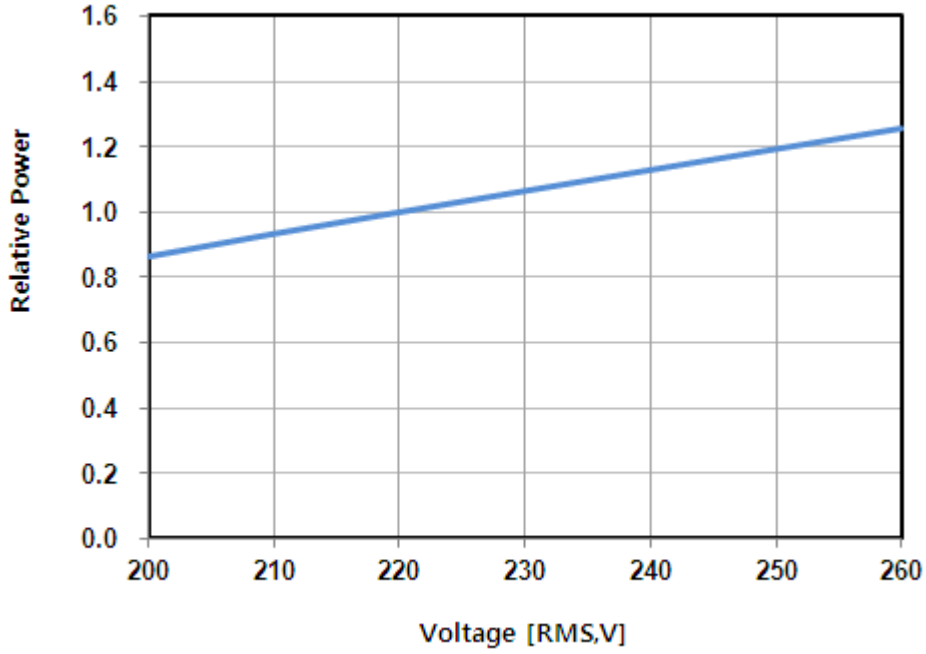
Fig 6. Relative Power Distribution vs. Voltage, T_a=25^{\circ}\text{C} , 220V
