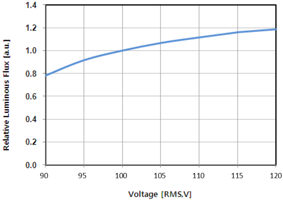
Fig 8. Relative Luminous Flux vs. Voltage at T_a=25^{\circ}\text{C} , 120V
