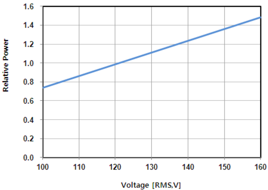
Fig 5. Relative Power Distribution vs. Voltage, T_a=25^{\circ}\text{C} , 120V
