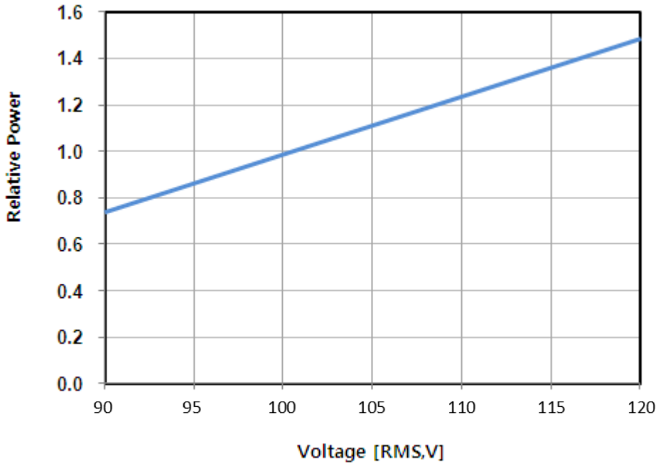
Fig 4. Relative Power Distribution vs. Voltage, T_a=25^{\circ}\text{C} , 100V
