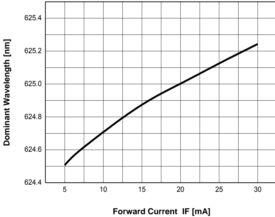
Fig 5. Dominant Wavelength vs. Forward Current, T_j = 25^\circ\text{C}
