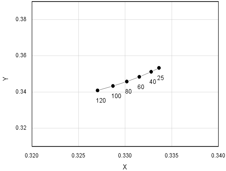
Fig 8. Chromaticity Coordinate vs. Junction Temperature I_F=40mA (4200K~7000K)
