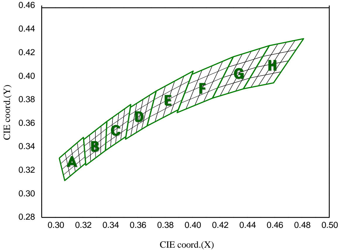
Fig 10. CIE Chromaticity Diagram T_a=25^\circ\text{C} , I_F=40\text{mA}
