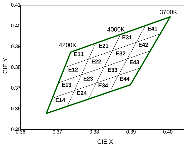
CIE Chromaticity Diagram (Neutral white), T_j=25^{\circ}\text{C} , I_F=60\text{mA}
