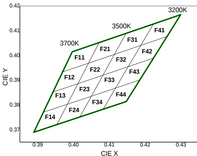
CIE Chromaticity Diagram (Warm white), T_j=25^{\circ}\text{C} , I_F=60\text{mA}
