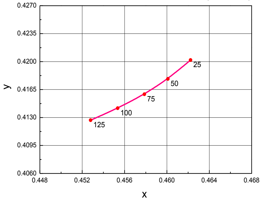
Fig 8. Chromaticity Coordinate vs. Junction Temperature, I_F=60\text{mA} (2600~4200K)
