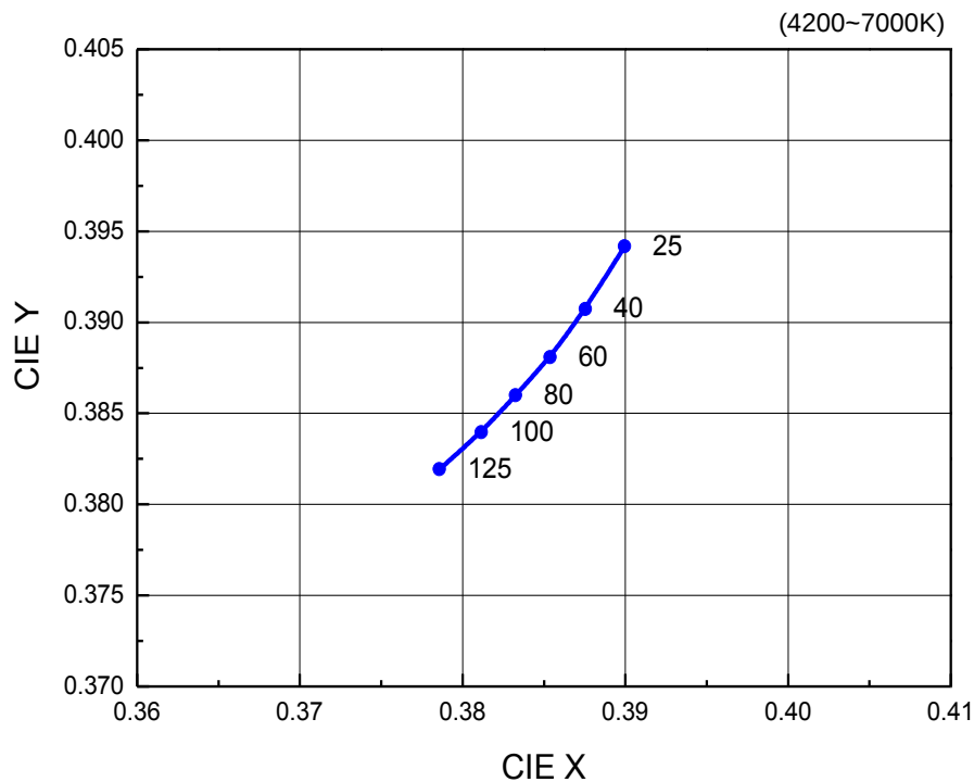
Fig 8. Chromaticity Coordinate vs. Junction Temperature, I_F=65\text{mA}
