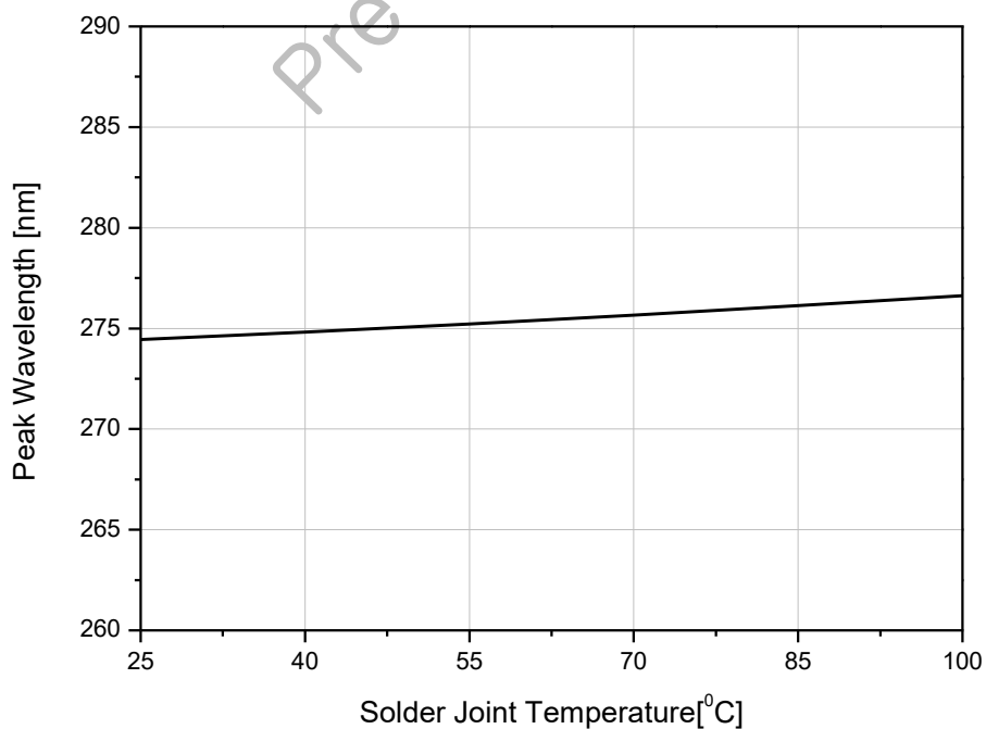
Fig 6. Solder Joint Temperature vs. Peak Wavelength, I_F=100\text{mA}
