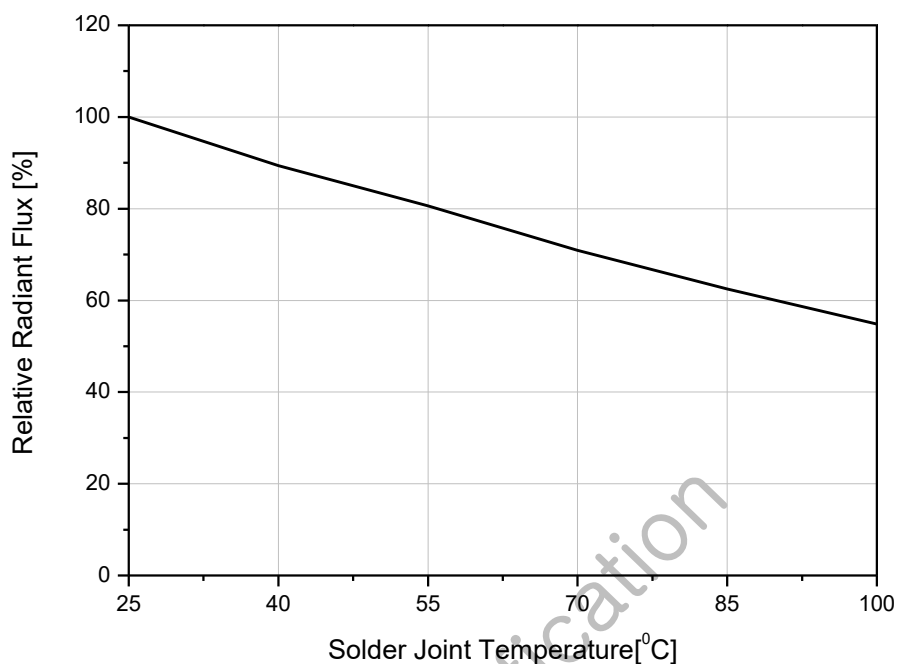
Fig 5. Solder Joint Temperature vs. Relative Radiant Flux, I_F=100\text{mA}
