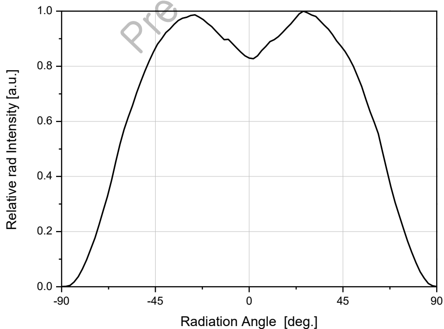
Fig 8. Typical Spatial Distribution, I_F=100\text{mA}
