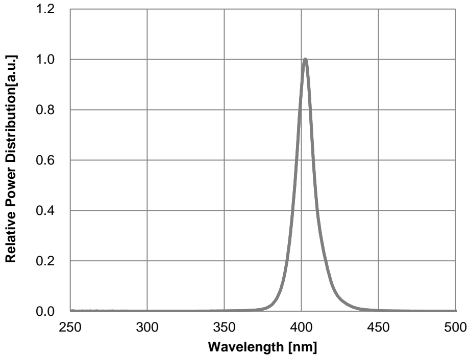
Fig 1. Spectrum, T_a=25^\circ\text{C} , I_F=9\text{A}
