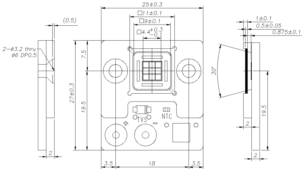
Screw View
