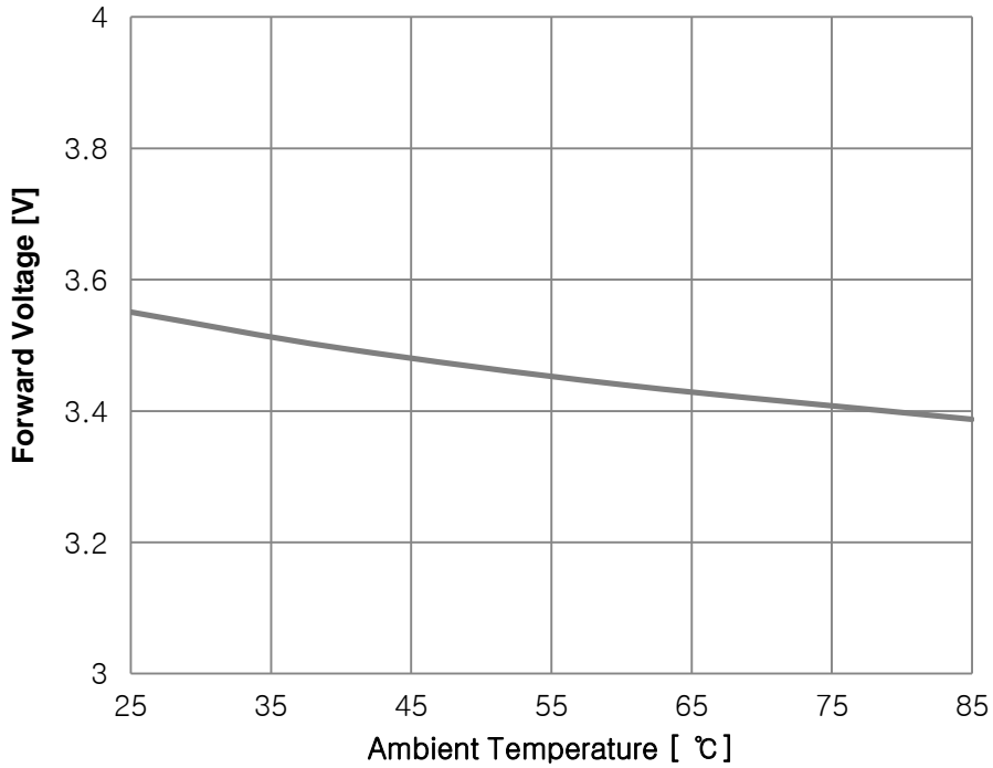
Fig 7. Ambient Temperature vs. Forward Voltage, I_F=9A
