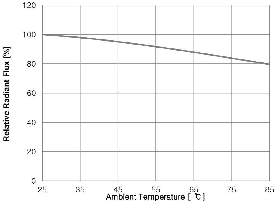
Fig 5. Ambient Temperature vs. Relative Radiant Flux, I_F=9A
