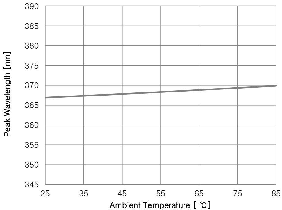
Fig 6. Ambient Temperature vs. Peak Wavelength, I_F=16A
