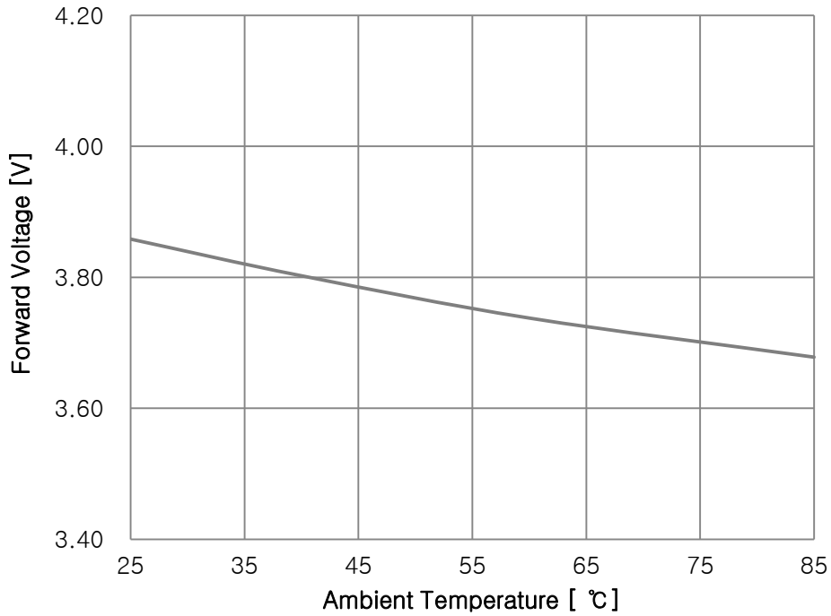
Fig 7. Ambient Temperature vs. Forward Voltage, I_F=16A
