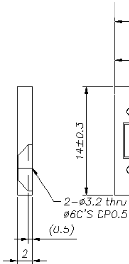
Screw Hole
