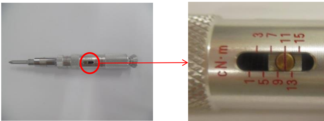
< Torque driver >
