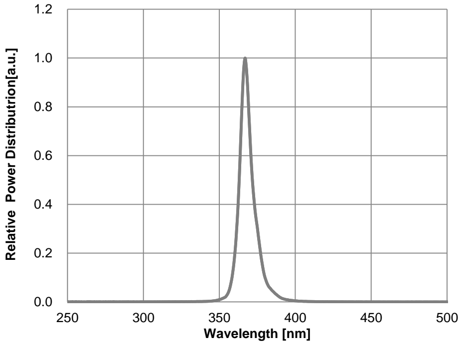
Fig 1. Spectrum, T_a=25^\circ\text{C} , I_F=16\text{A}
