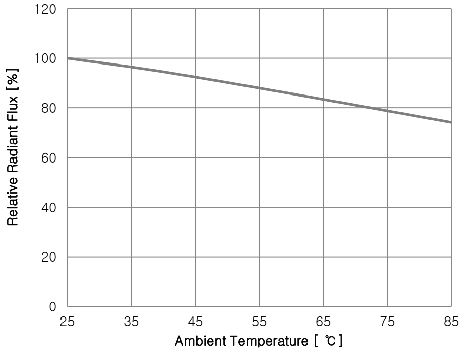
Fig 5. Ambient Temperature vs. Relative Radiant Flux, I_F=16A
