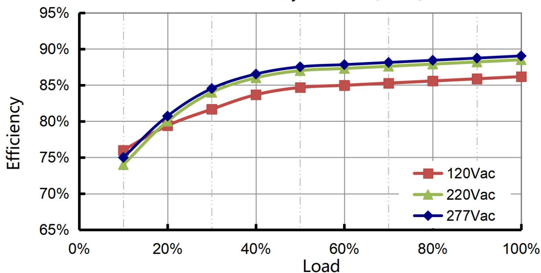
Efficiency vs. Load (C280)
