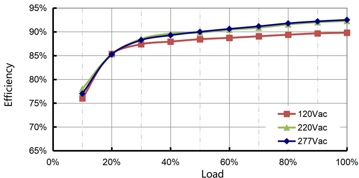
Efficiency vs. Load (C070)
