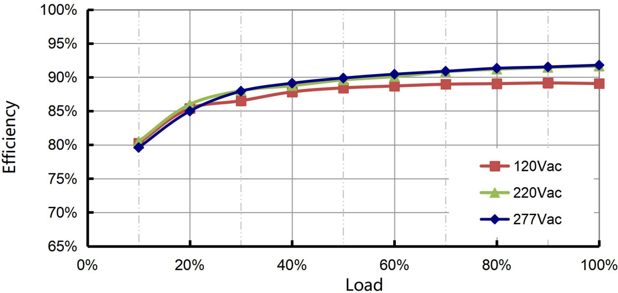
Efficiency vs. Load (C105)
