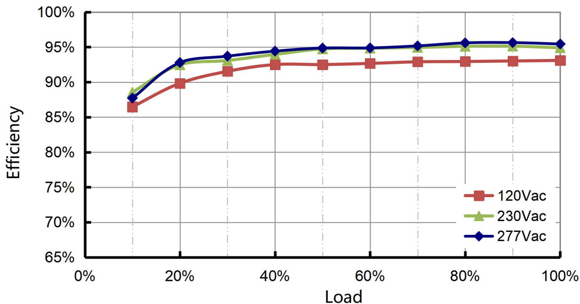
Efficiency vs. Load (C860)
