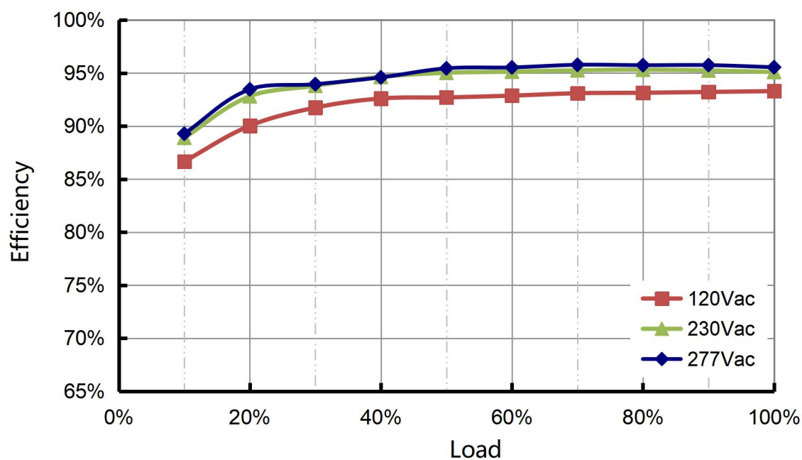
Efficiency vs. Load (C21A)
