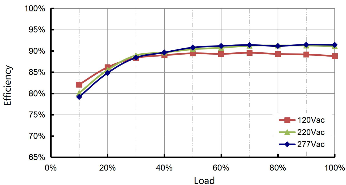
Efficiency vs. Load (C630)
