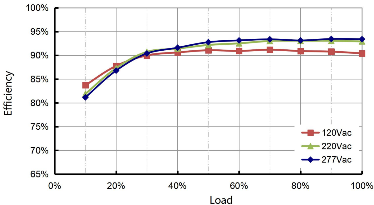
Efficiency vs. Load (C210)
