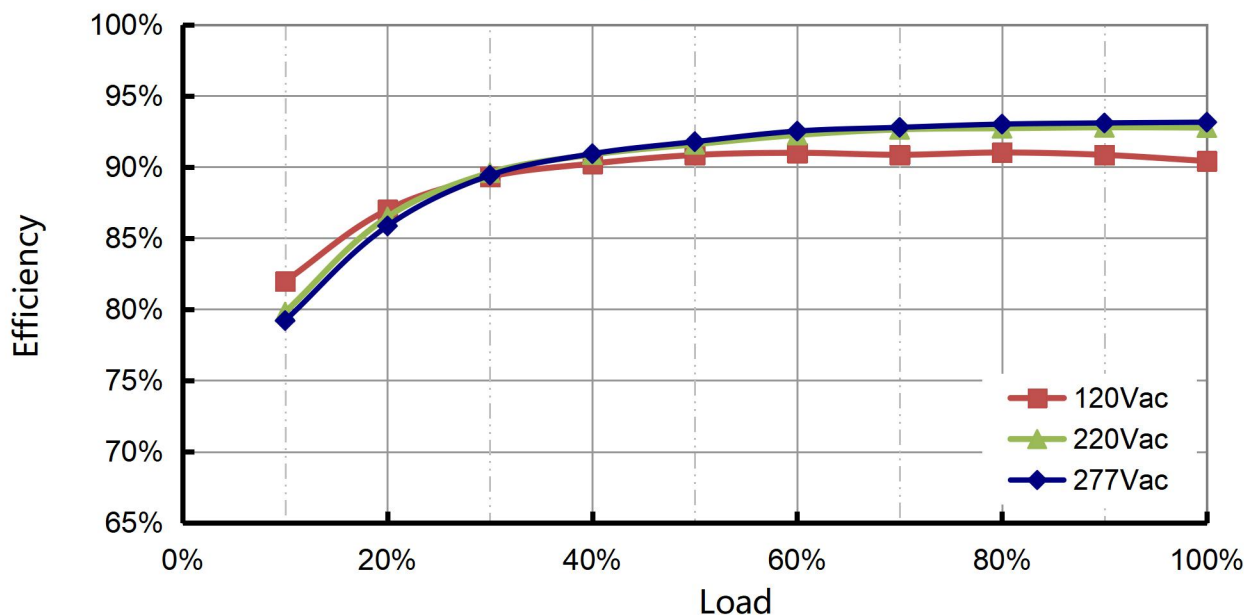
Efficiency vs. Load (C280)
