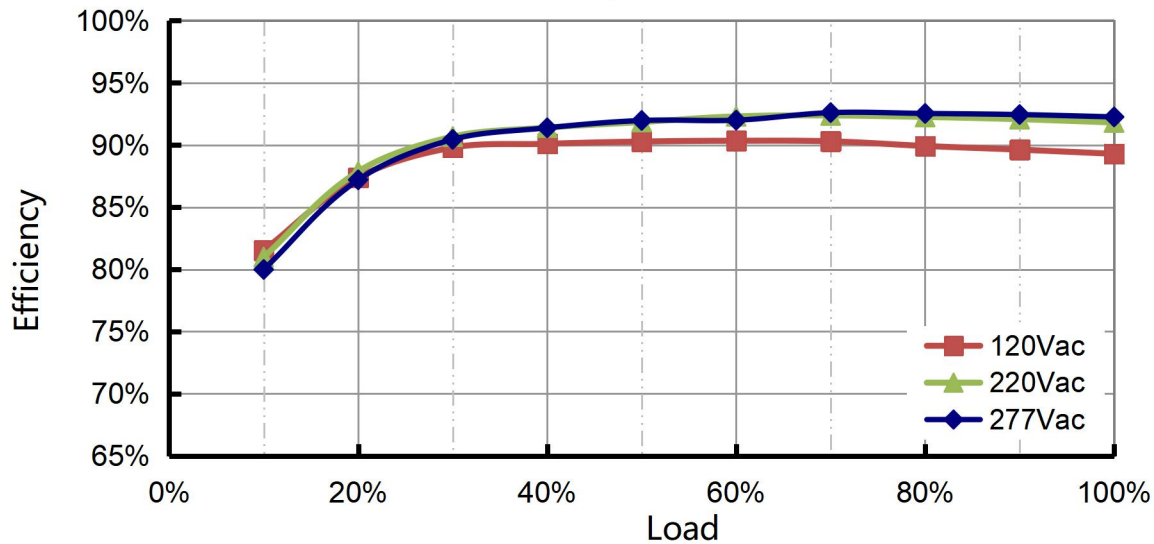
Efficiency vs. Load (C690)
