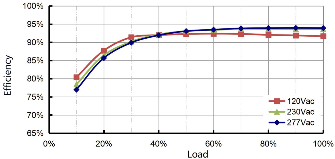
Efficiency vs. Load (C990)
