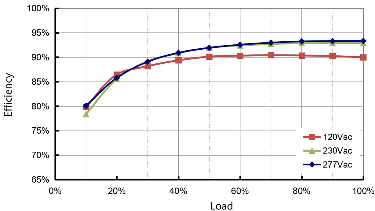
Efficiency vs. Load (C420)
