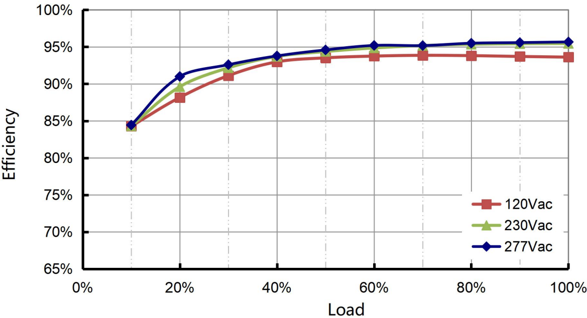
Efficiency vs. Load (C860)
