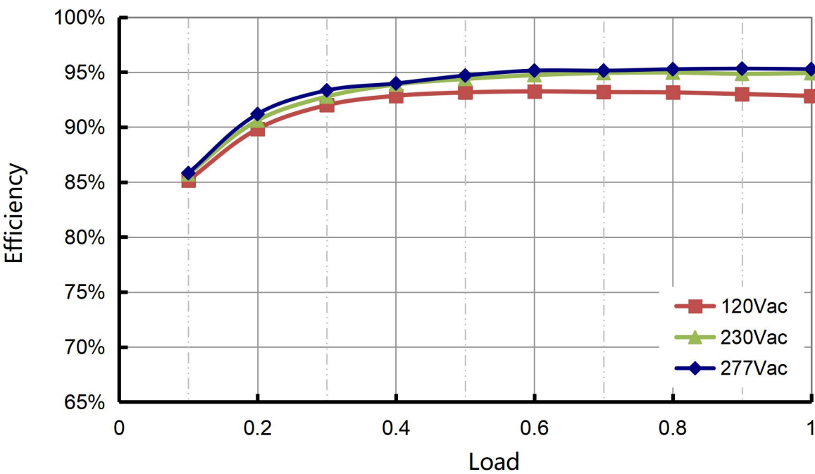
Efficiency vs. Load (C16A)
